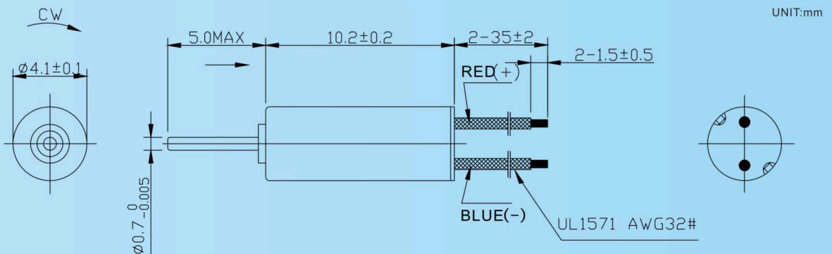
Model: 0410RN04-30M-35
