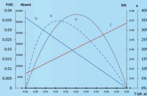
Model: 0410RN04-30M-35
