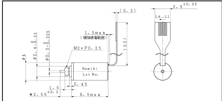
For combination with gearhead: SPG04
