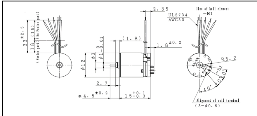
For combination with gearhead: SSG12, SPG12
