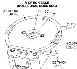
R-OPTION BASE (ROTATIONAL MOUNTING)
